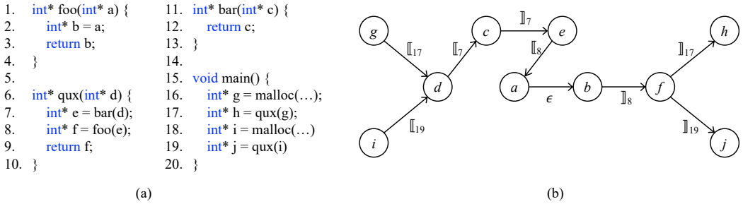
Fig. 1. The value-flow graph of the code snippet. The edges, (u, v) , labeled by \llbracket_{\kappa} and \rrbracket_{\kappa} represent assignments from the variable u to the variable v via function call and function return at Line \kappa , respectively. An edge labeled by \epsilon represents an intra-procedural assignment.
