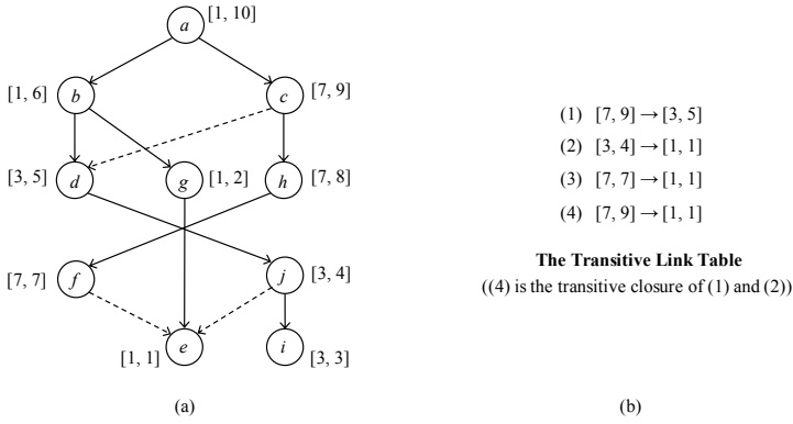
Fig. 12. (a) A graph where one of its spanning trees is represented by the solid edges and non-tree edges are the dashed edges. Vertices are labeled by intervals for reachability queries. (b) The transitive link table for encoding reachability relations implied by the non-tree edges.
