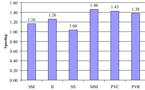
Figure 9. Performance speedup of co-processing on the CPU and the GPU over processing on the GPU only.
