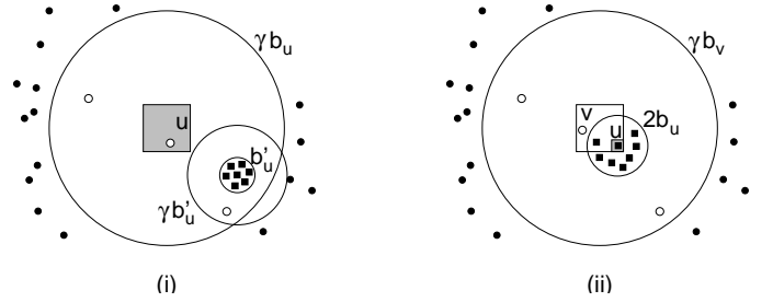
Figure 1: The separation properties for (i) type-2 cells satisfying property (a) and (ii) type-3 cells. Pollutants are indicated with hollow circles and points of the inner clusters are shown as black squares.
