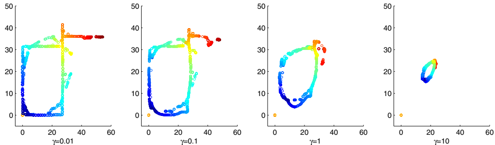
Figure 8. The impact of \gamma on co-embedding. We use the “co-embedding with location constraints” method. We can see that with a small \gamma (left plot), the relative weight of the location constraints is large, hence the source training data are embedded almost “right at” their ground truth locations. With increasing \gamma , the location constraints gradually fade out. Note that in all these 4 figures, there are some (overlapping, in warm color) data points located at location (0,0). They are actually the target training data from the right-wing hallway (warm color), and are embedded in a wrong location because there is no Maximal-RSS correspondence found in the right wing hallway between dataset 1 and 2, as shown in Figure 4’s left plot.
