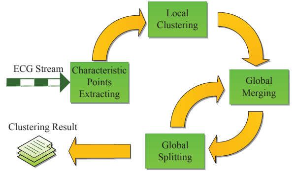
Fig. 2. Algorithm overview.
