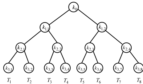
Fig. 1. A binary key tree with eight tags
