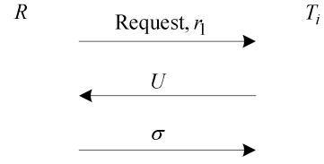
Fig. 4. Authentication Procedure in LAST. Upon U , \mathcal{R} 's operations are: 1. authenticating \mathcal{T}_i and key-updating; 2. computing \sigma and sending it to \mathcal{T}_i . \mathcal{T}_i also updates its keys after checking \sigma .
