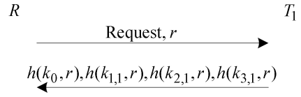
Fig. 3. A basic authentication procedure of tree-based approaches
