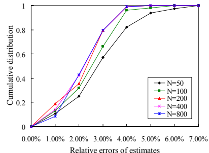
Figure 17. Estimation accuracy with different sample sizes
