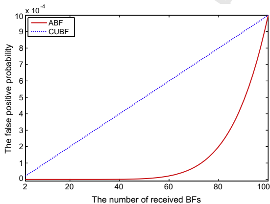
Fig. 8. The false positive probability of CUBF and ABF as functions of the number of BFs, where \sigma = 0.001 , n = 30 , s = 100 , and the parameters m and k are optimized by Formulas (4)–(7).
