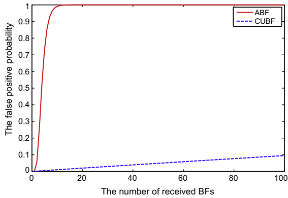
Fig. 7. f_{CUBF} and f_{ABF} are functions of the number of received BFs, where f_{BF} = 0.001 , m/n = \log_{0.6185} 0.001 , and k = (m/n) \ln 2 .
