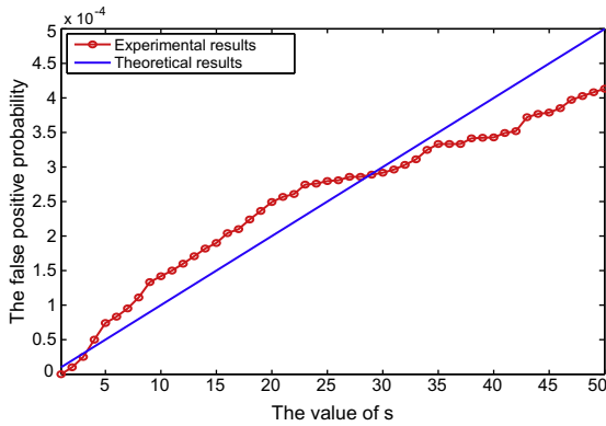
Fig. 14. The theoretical and experimental values of f_{CUBF} as functions of the number of BFs, where \sigma = 0.001 , n = 30 , m and k are optimized by Formulas (4)–(7).
