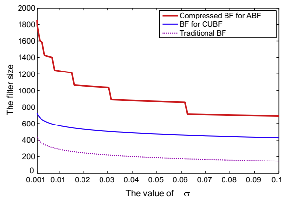
Fig. 9. The sizes of traditional BF, BF for CUBF, and compressed BF for ABF as functions of \sigma , where s = 100 and n = 30 .
