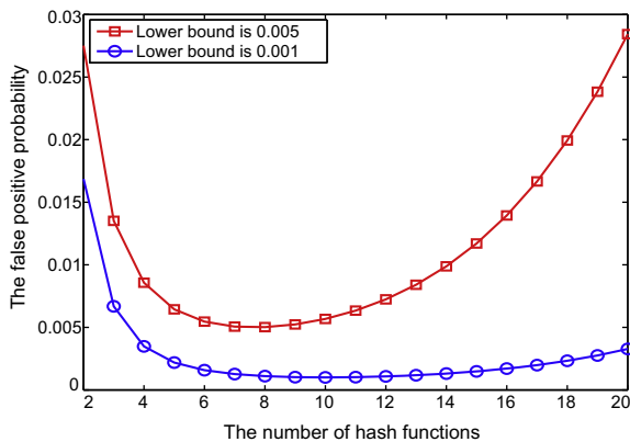
Fig. 5. The false positive probability of CUBF as a function of the number of hash functions used, where s = 100 and n = 30 .
