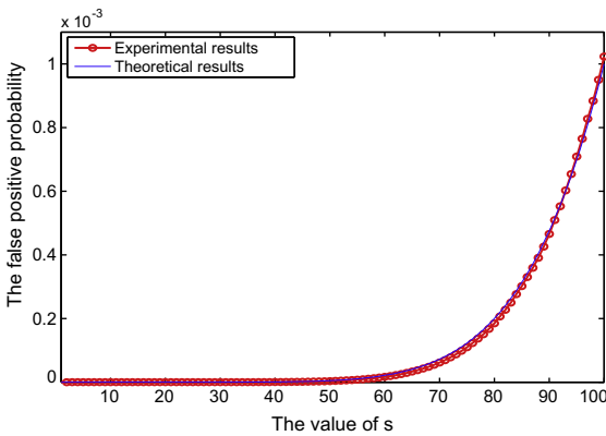
Fig. 15. The theoretical and experimental values of f_{ABF} as functions of the number of BFs, where \sigma = 0.001 , n = 30 , and the parameters m and k are optimized by Formulas (4)–(7).
