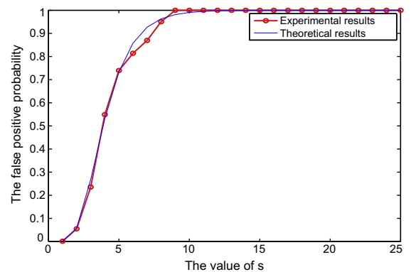
Fig. 13. The theoretical and experimental values of f_{ABF} as functions of the number of BFs. For each single BF, the false positive probability is 0.001, m/n = \log_{0.6185} 0.001 , and k = (m/n) \ln 2 .
