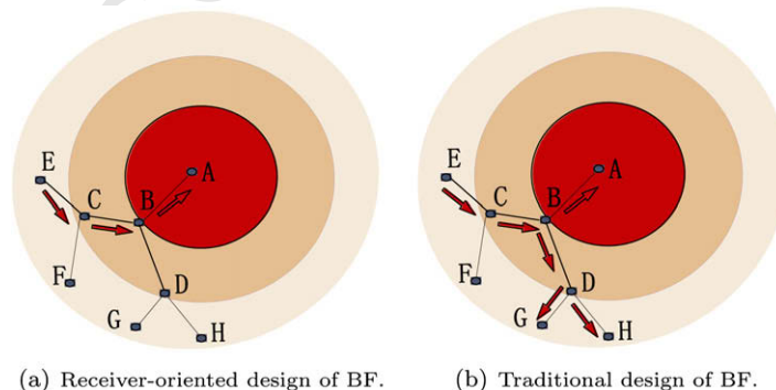
Fig. 1. Illustrative examples of BF-based routing for a query for an item at node A.
