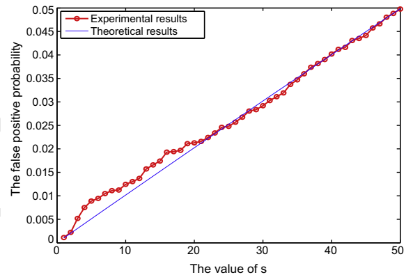
Fig. 12. The theoretical and experimental values of f_{CUBF} as functions of the number of BFs. For each single BF, the false positive probability is 0.001, m/n = \log_{0.6185} 0.001 , and k = (m/n) \ln 2 .
