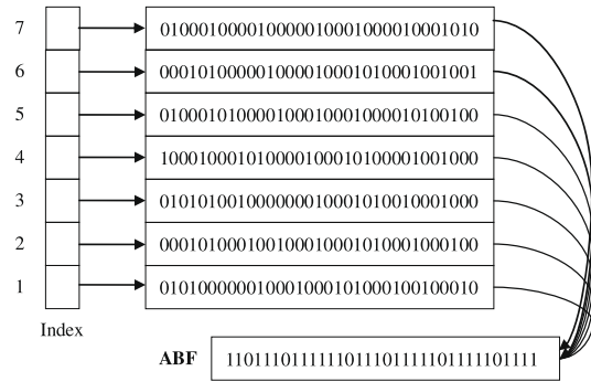
Fig. 3. An example of an ABF based on seven BFs, where m = 33 , n = 3 , k = 3 , and f_{BF} = 0.0136 . Note that the false positive probability of the resulting ABF is f_{ABF} = 0.618 .
