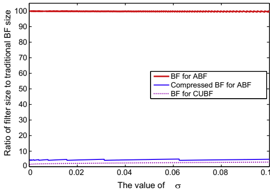
Fig. 10. The ratio of filter size to the traditional BF size as function of \sigma , where s = 100 and n = 30 .
