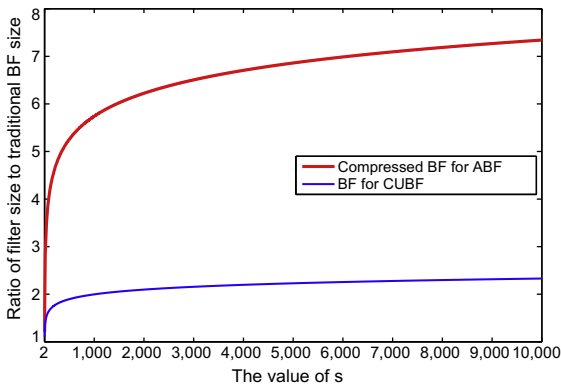
Fig. 11. The ratio of filter size to the traditional BF size as functions of s , where \sigma = 0.001 and n = 30 .
