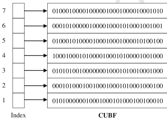
Fig. 2. An example of a CUBF consisted of seven BFs, where m = 33 , n = 3 , k = 3 , and f_{BF} = 0.0136 . Note that the false positive probability of the resulting CUBF is f_{CUBF} = 0.0914 .
