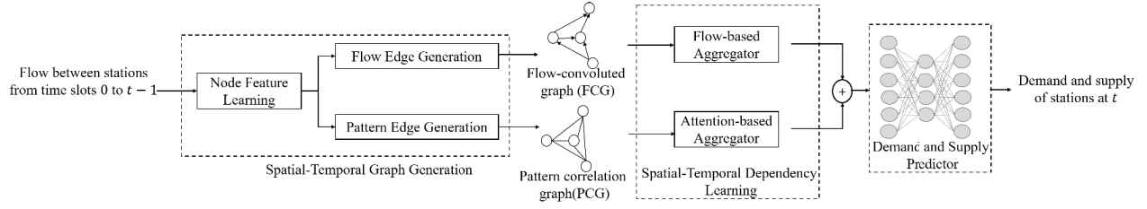
Fig. 1. Overview of STGNN-DJD.
