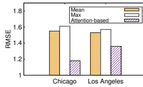
(a) RMSE.
