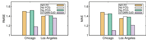
(a) RMSE.
