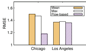
(a) RMSE.
