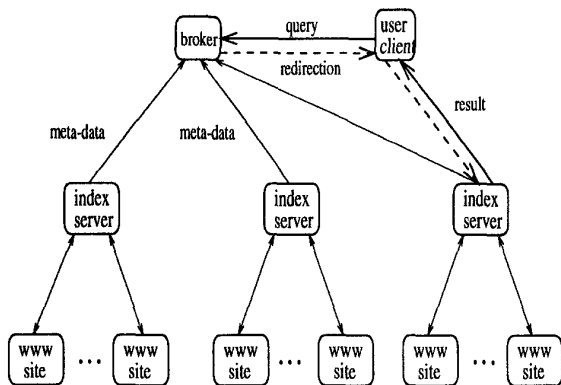
Figure 1: Multiserver organization and query routing.
