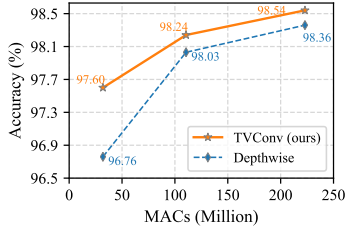
(b) ShuffleNetV2 as the architecture
