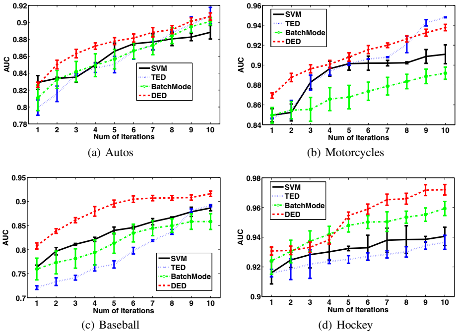
Fig. 1. Learning curves for four binary classification tasks on Newsgroups data
