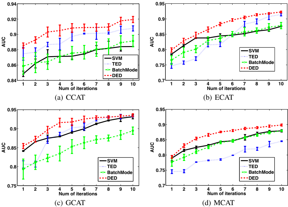
Fig. 2. Learning curves for four binary classification tasks on Reuters data
